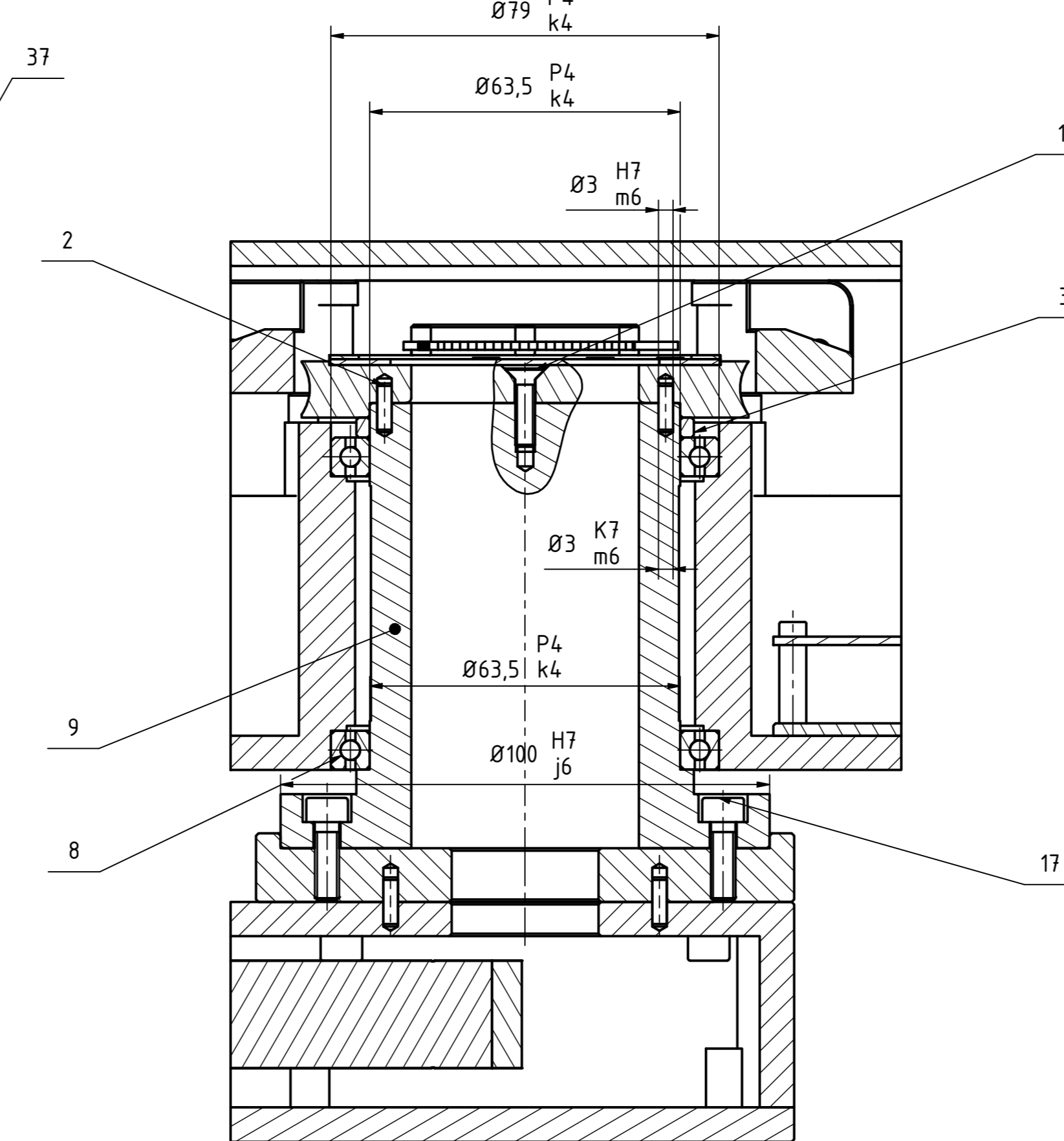
B-B (1:1)
