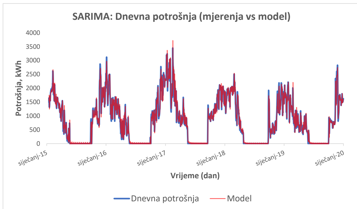
Slika 6.9 SARIMA model (3, 1, 3)(0, 1, 1)_{12}
