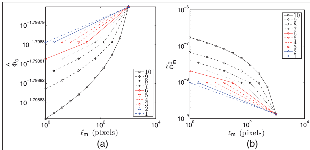
Figure 14. Change of (a) the dimensionless correlation residuals and (b) equilibrium residuals for different regularization lengths and different number of jumps (indicated in the legend) to decrease the regularization length. Note the narrow range of variation of \hat{\Phi}_c .
