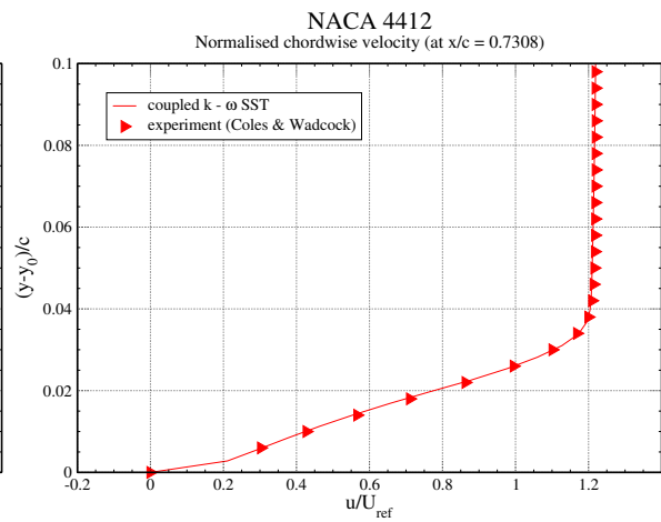
(b) x/c = 0.7308 ,
