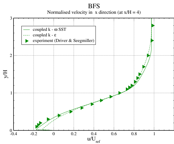
(c) x/H = 4 ,
