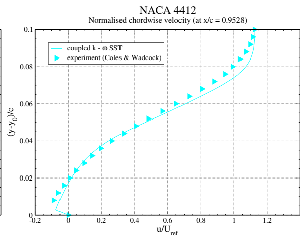
(f) x/c = 0.9528 .
