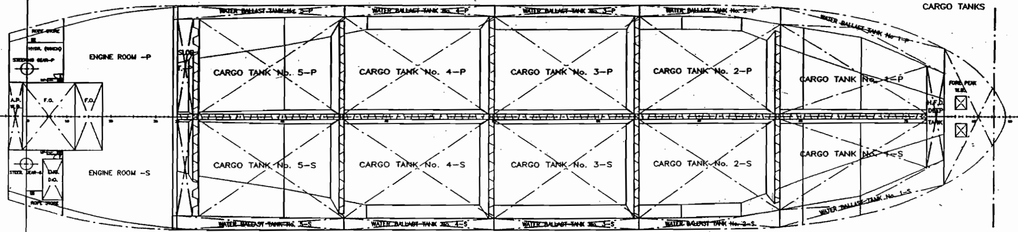
CARGO TANKS
