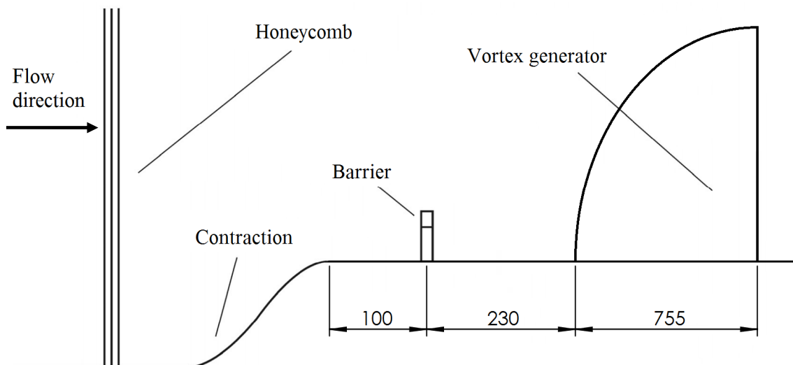
Figure 3.11 Arrangement of the castellated barrier wall and vortex generators in the CET climatic wind tunnel, dimensions are given in mm
