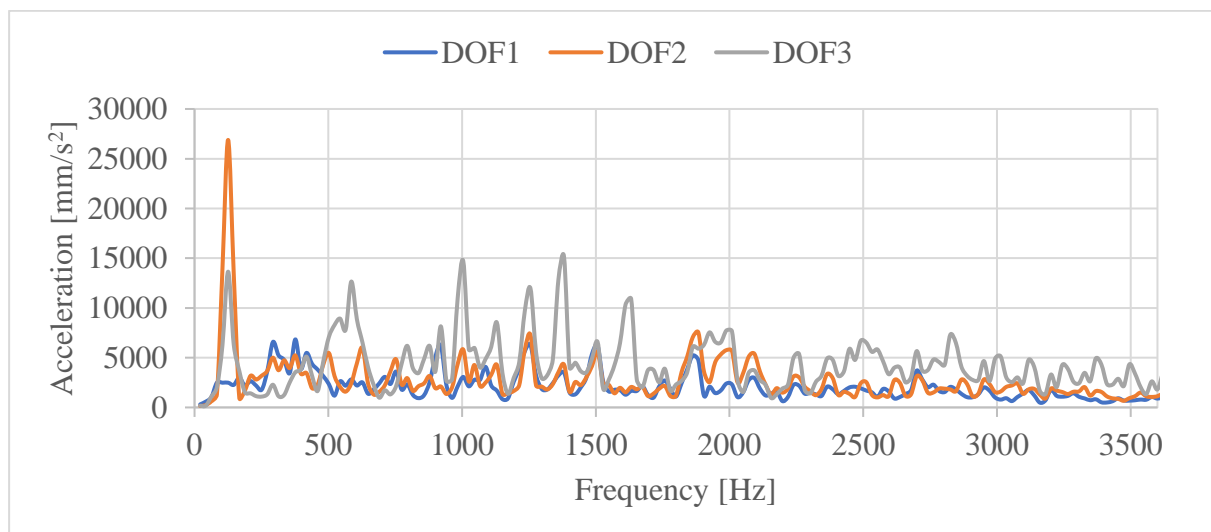
Figure 29. Averaged excitation
