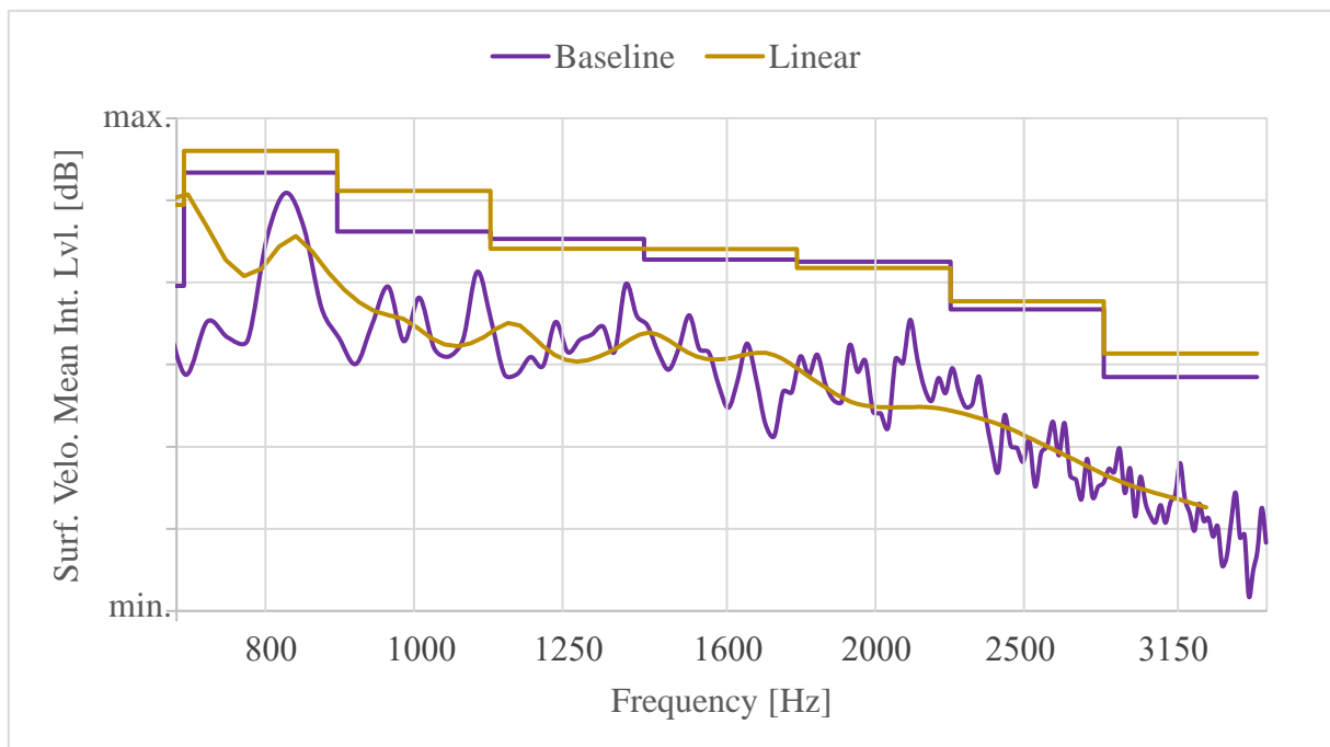
Figure 50. Structure response comparison between baseline and linear excitation
