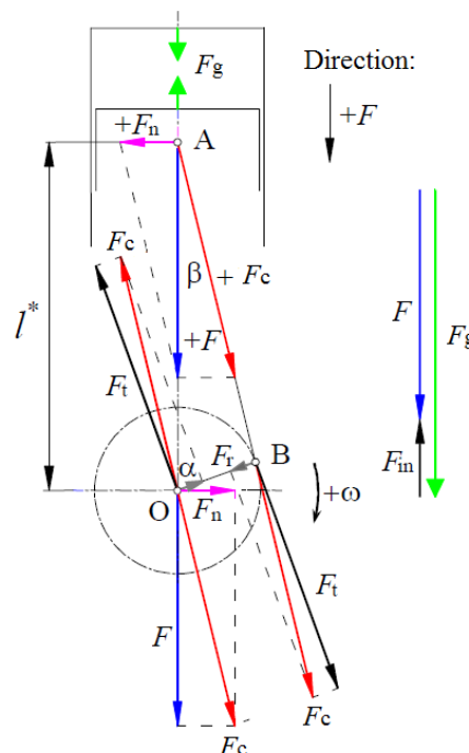
Figure 3. Cylinder forces [11]
