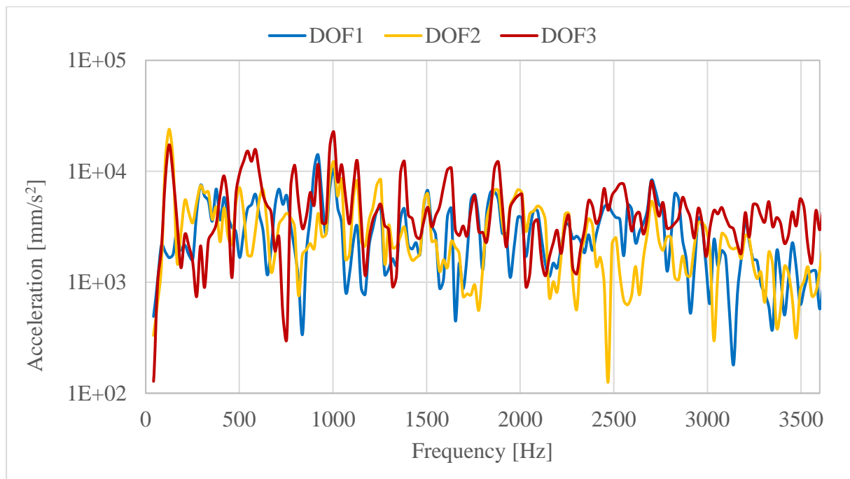
Figure 20. Acceleration in frequency domain in semi-logarithmic scale at node 5000405
