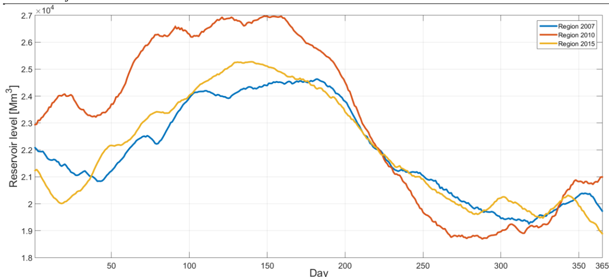
Figure 6.3. Annual, region aggregated, reservoir level for dry (2007), average (2015) and wet (2010) year in Mm 3 as results from the MTHC model
