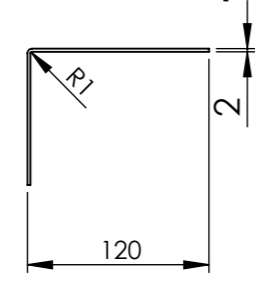
A (M1:5)
