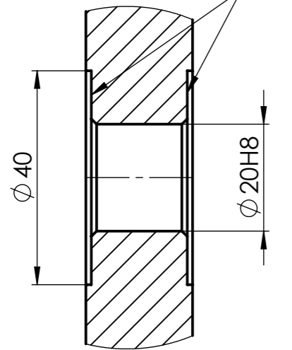
DETAILJ C M1:1
