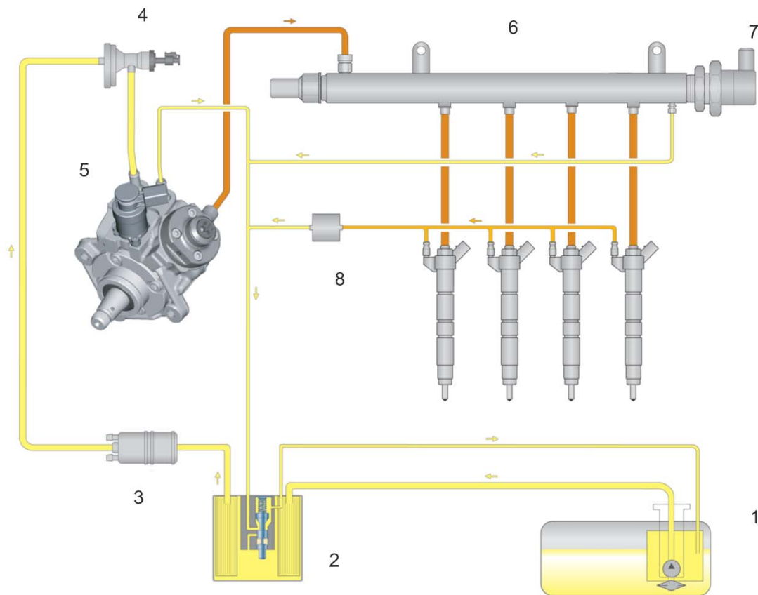
Figure 10. Fuel system [17]
