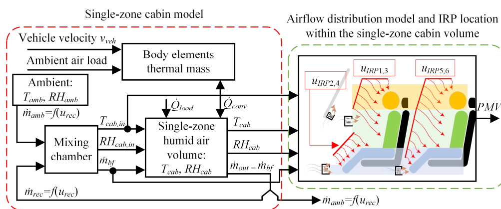
Figure 2. Block diagram of cabin thermal system model including airflow distribution model used for Predicted Mean Vote (PMV) evaluation.
