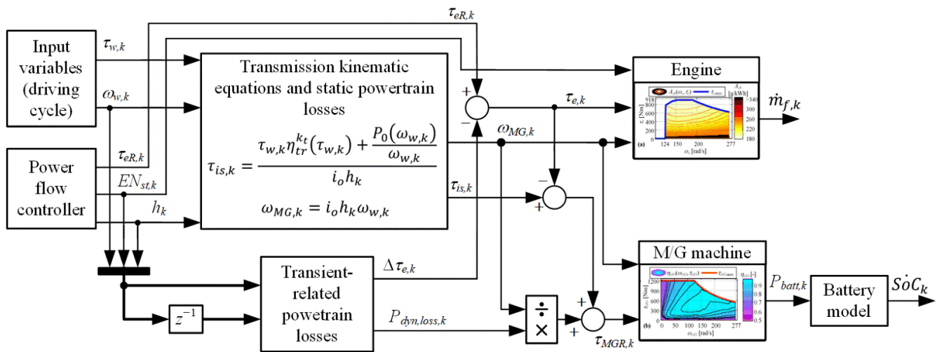
Figure 13. Block diagram of extended backward (EXT-BWD) model.
