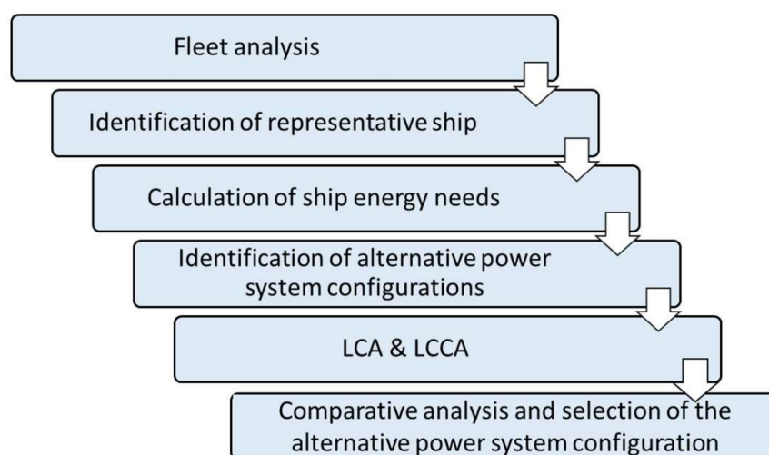
Figure 1. Procedure for the selection of alternative power systems configuration for inland waterway vessels.
