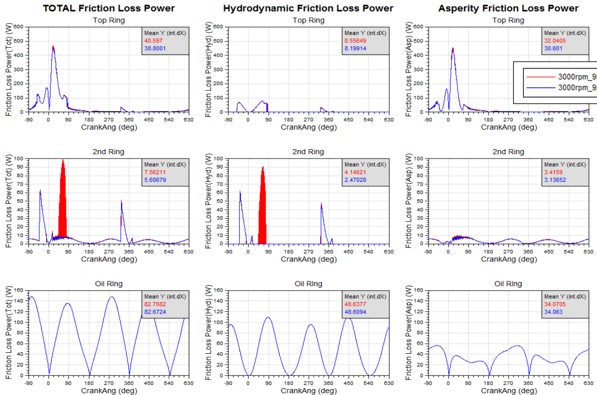
Figure B. 3. Comparison between BASIC and LOW FT ring package - Friction Power Loss overview.
