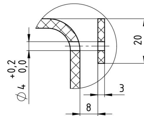
F(1:1)
