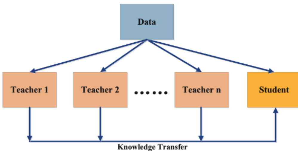
Slika 11. Multi-Teacher Distillation [10]
