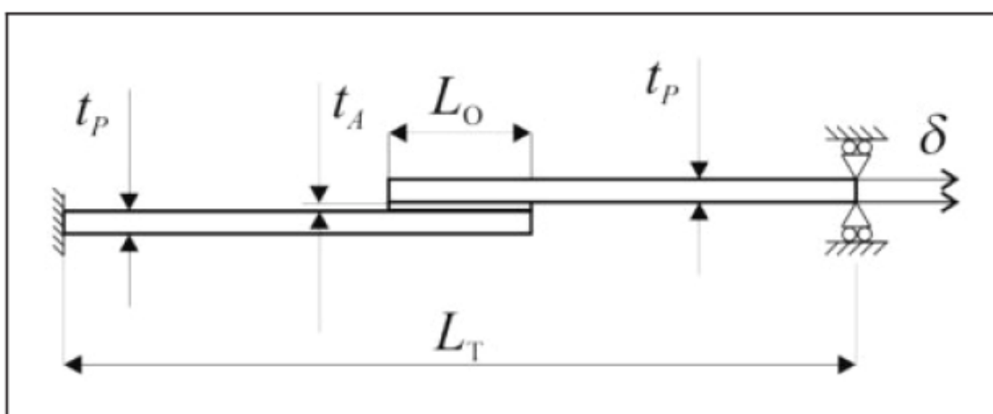
Figure 21. Schematic view of geometry and characteristic dimensions of SLJ [15]
