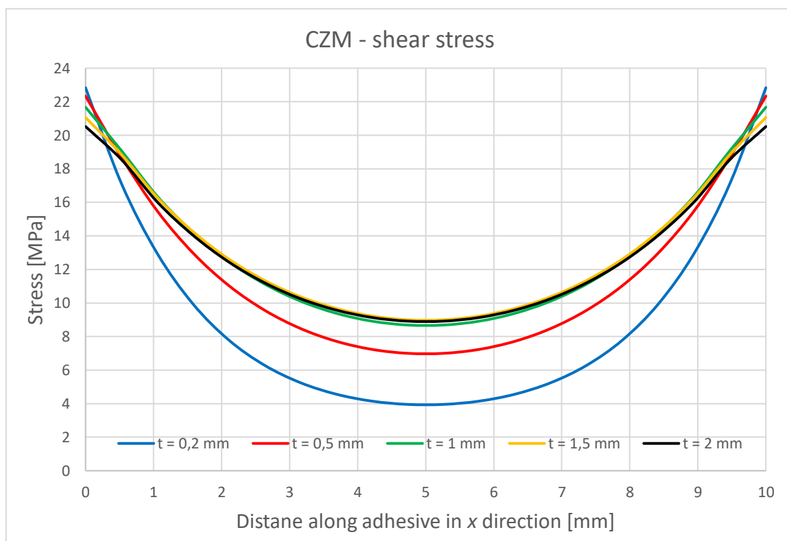
Figure 78. Distribution of shear stress within adhesive for different bondline thicknesses for CZM model
