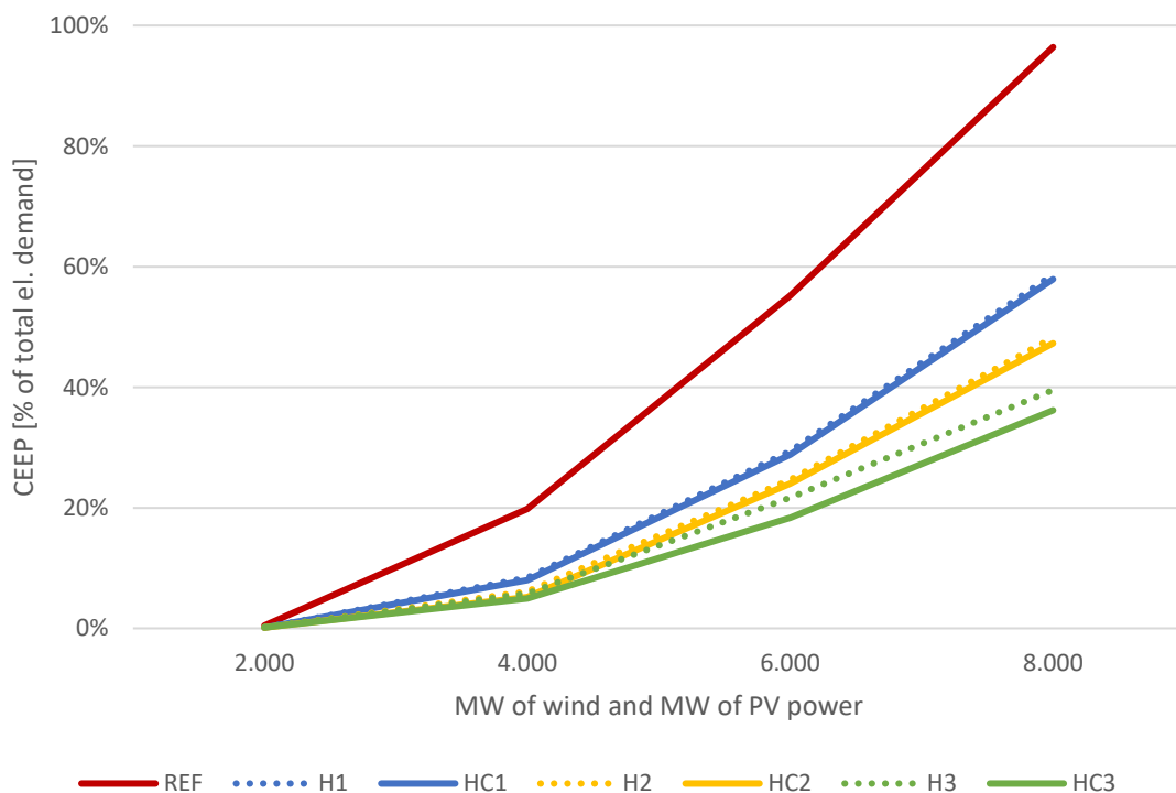
318 Figure 4 CEEP for all scenarios with electrical boiler limit of 2.500 MW
