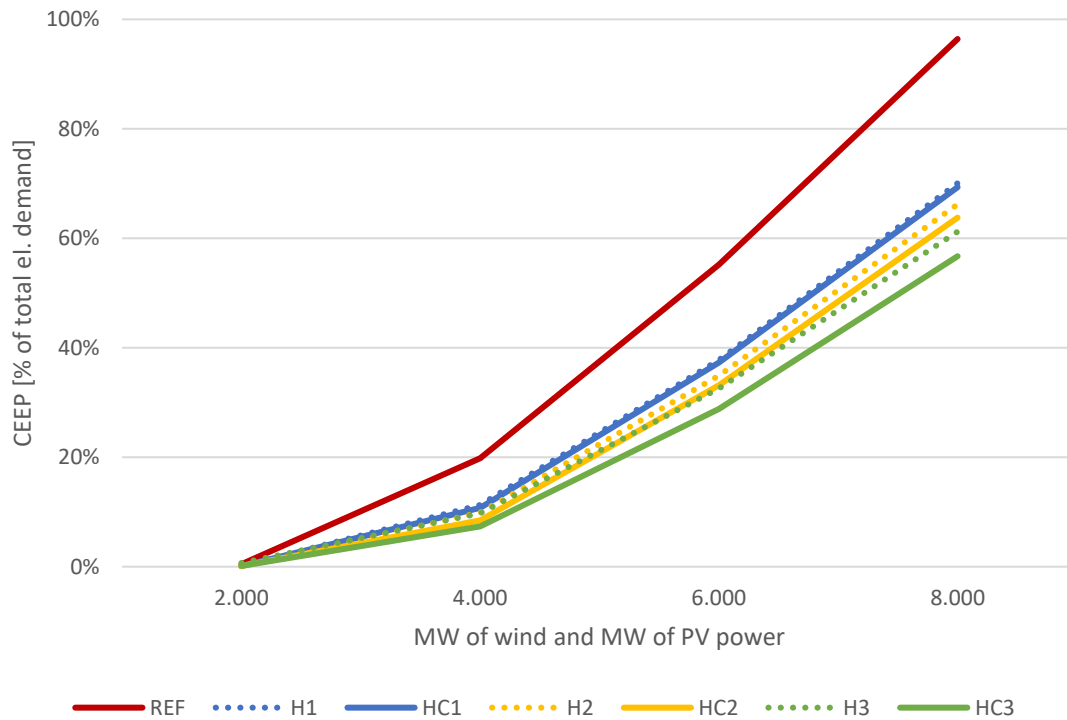
316 Figure 3 CEEP for all scenarios with electrical boiler limit of 600 MW
