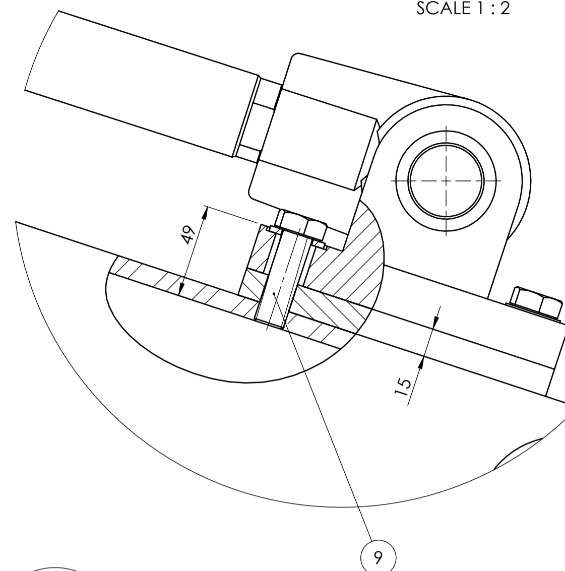
DETAIL H SCALE 1:2
