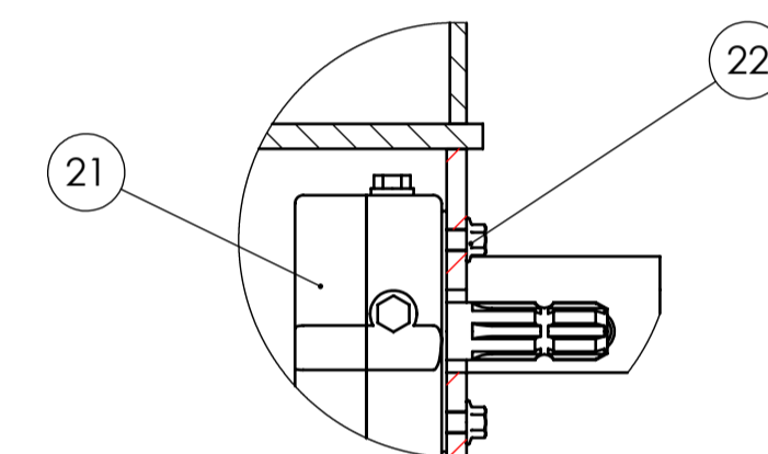
DETAIL I SCALE 1:5
