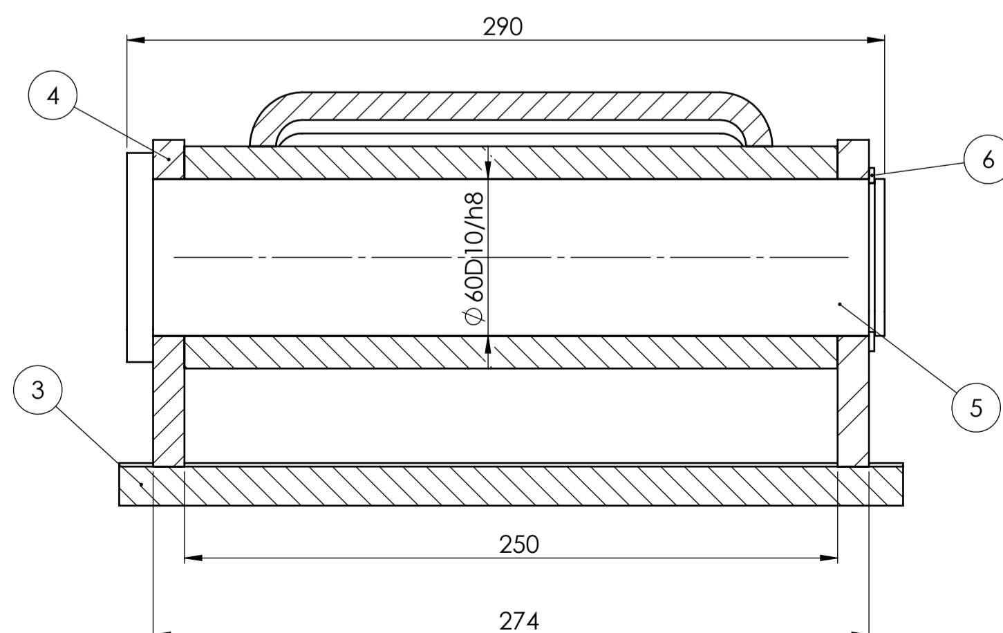
SECTION C-C SCALE 1:2
