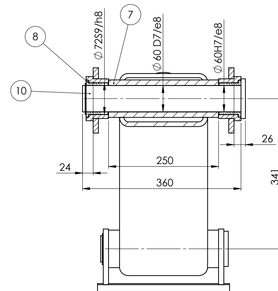
SECTION G-G SCALE 1:5
