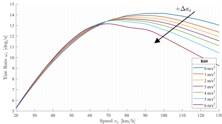
Figure 19. Positive longitudinal acceleration influence on yaw rate reference – constant steering angle at the beginning of R60 acceleration in turn manoeuvre
