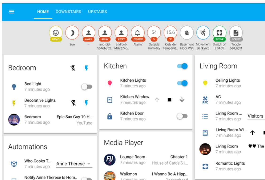
Slika 17. Home Assistant
