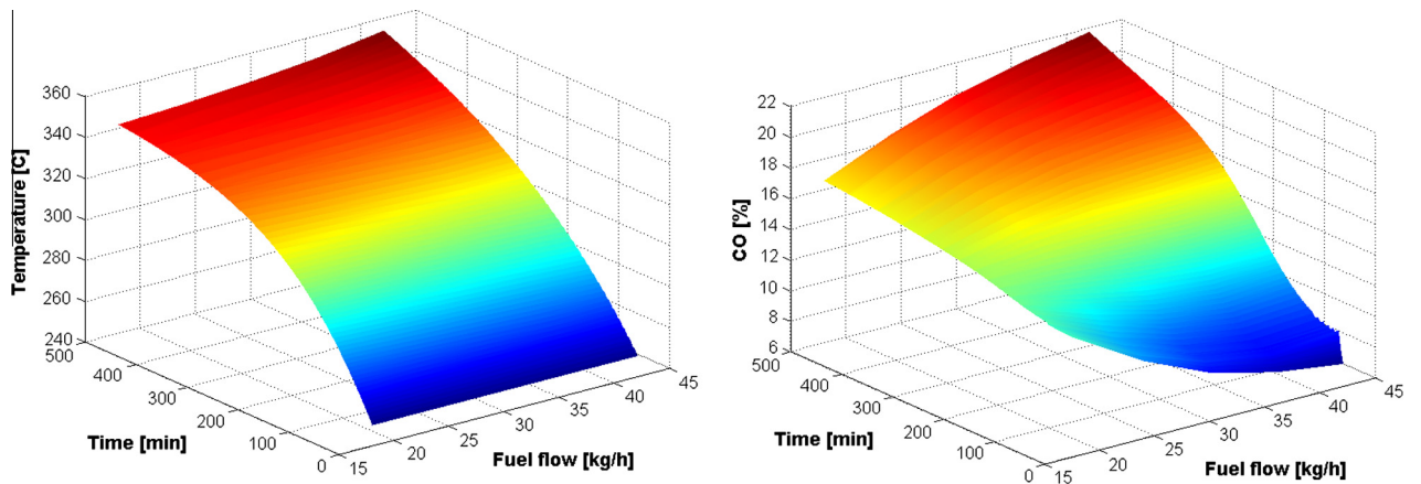
Fig. 17. Process analysis with the fuel flow changes.
