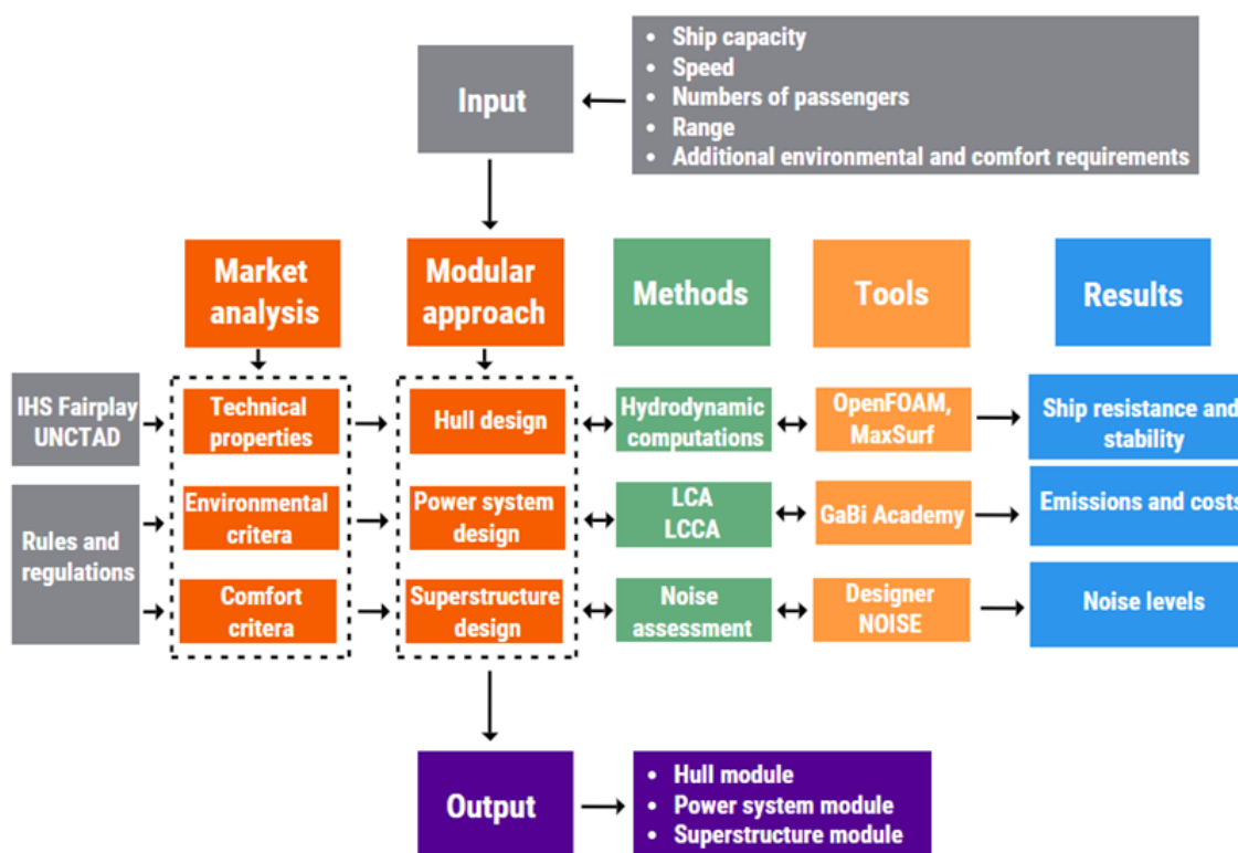
Figure 22. The ship design procedure based on the modular concept [105]
