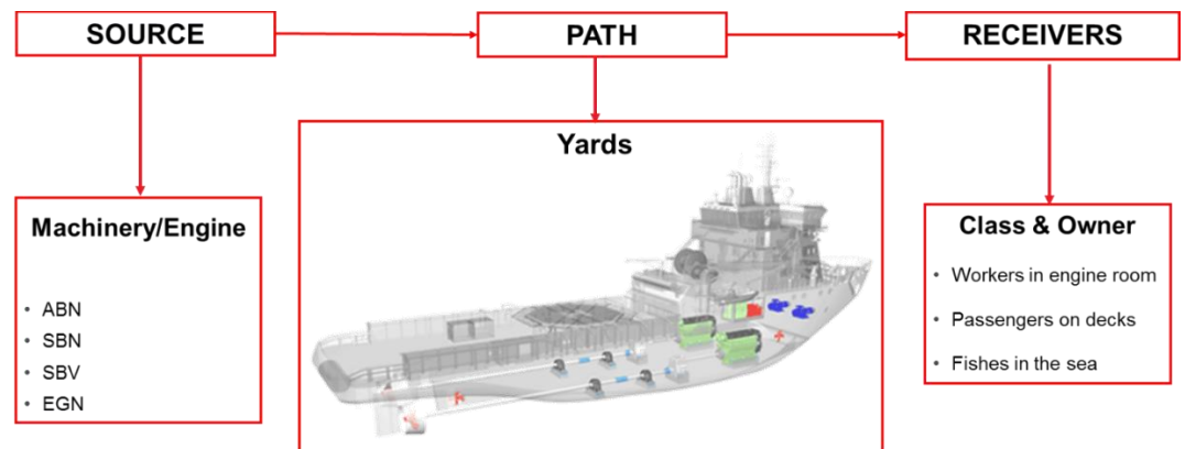
Figure 9. Source-Path-Receiver model
