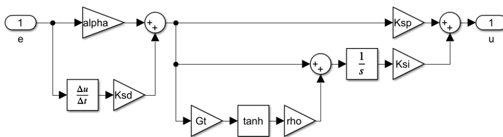
Slika 65. Model SMC-PID regulatora
