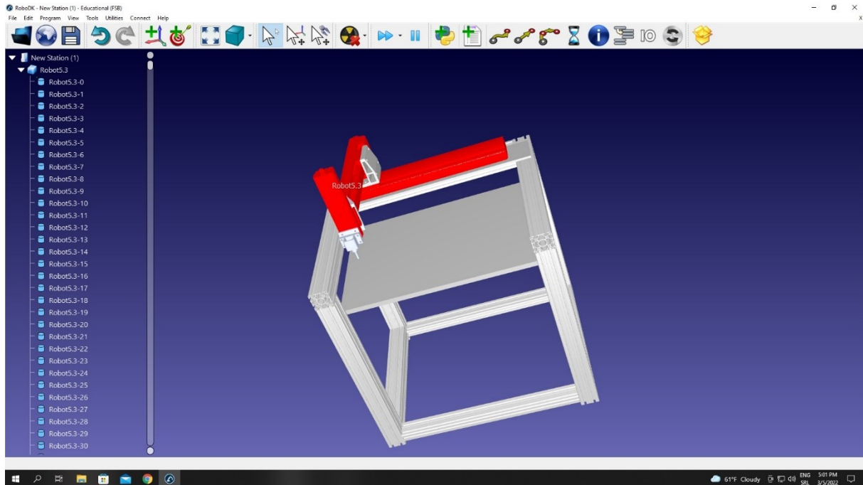
Slika 31. Model robota u programu RoboDK nakon naredbe split
