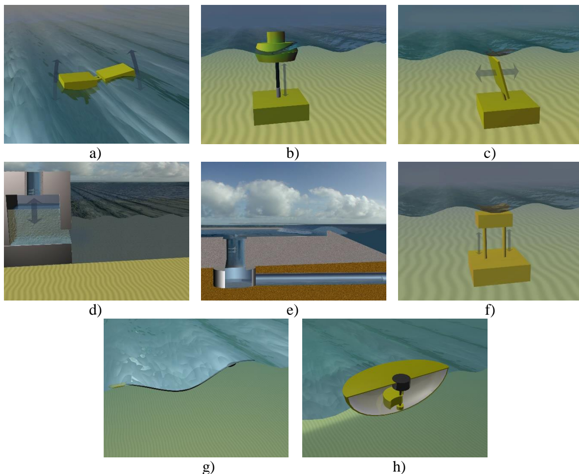
Figure 10. Types of wave energy converters [45]
