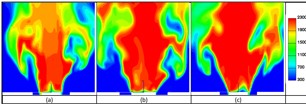
Figure 49 - Flame PSF30: qualitative difference in fields of temperature between C_s=f (CSM) (a), C_s=0.1 (b) and C_s=0.2 (c)
