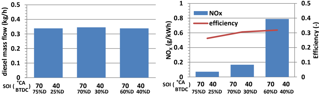
Figure 111. Optimization of diesel fuel quantities
