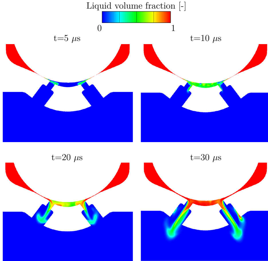
Figure 4.6: Standard Spray G liquid phase volume fraction at the early stage of injection
