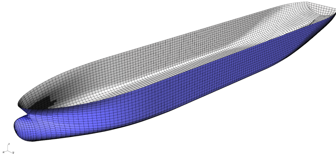
Figure 5 Hydrodynamic panel model of the intact tanker.
