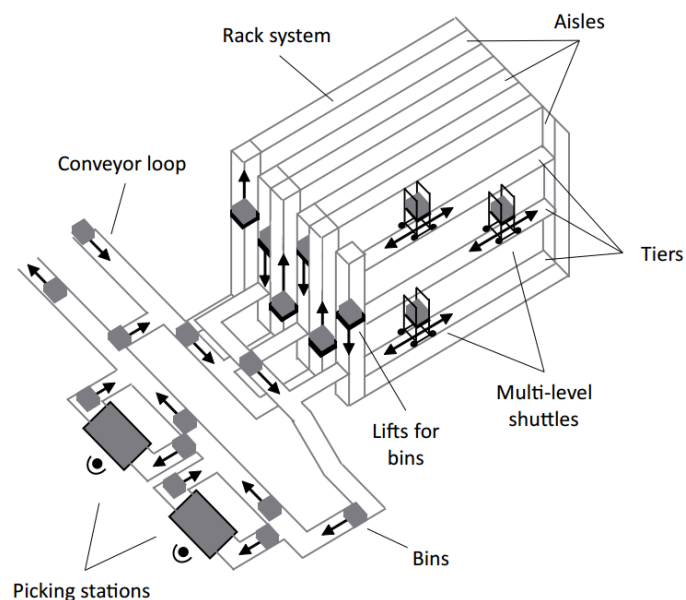
Slika 13. Multi-level SBS/RS [20]
