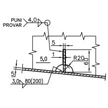
DETALJ "2": M 1:5
