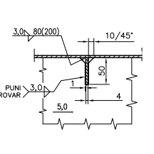
DETALJ "4": M 1:5
