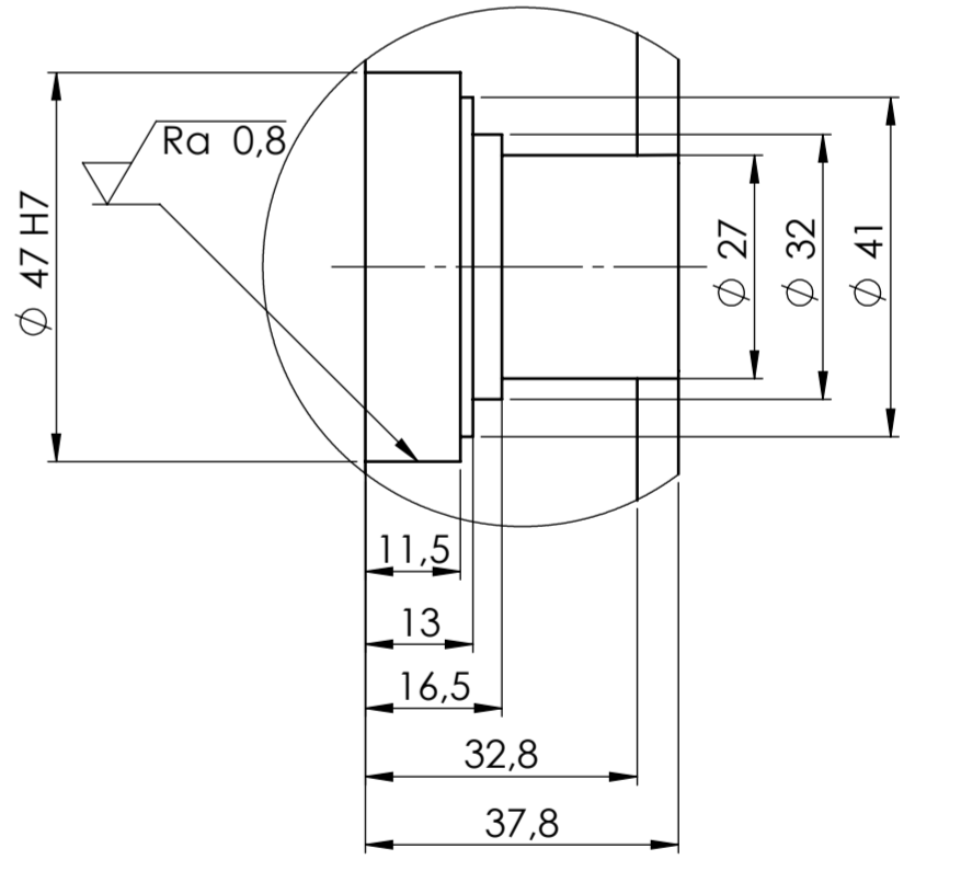
DETALJ D (1:1)
