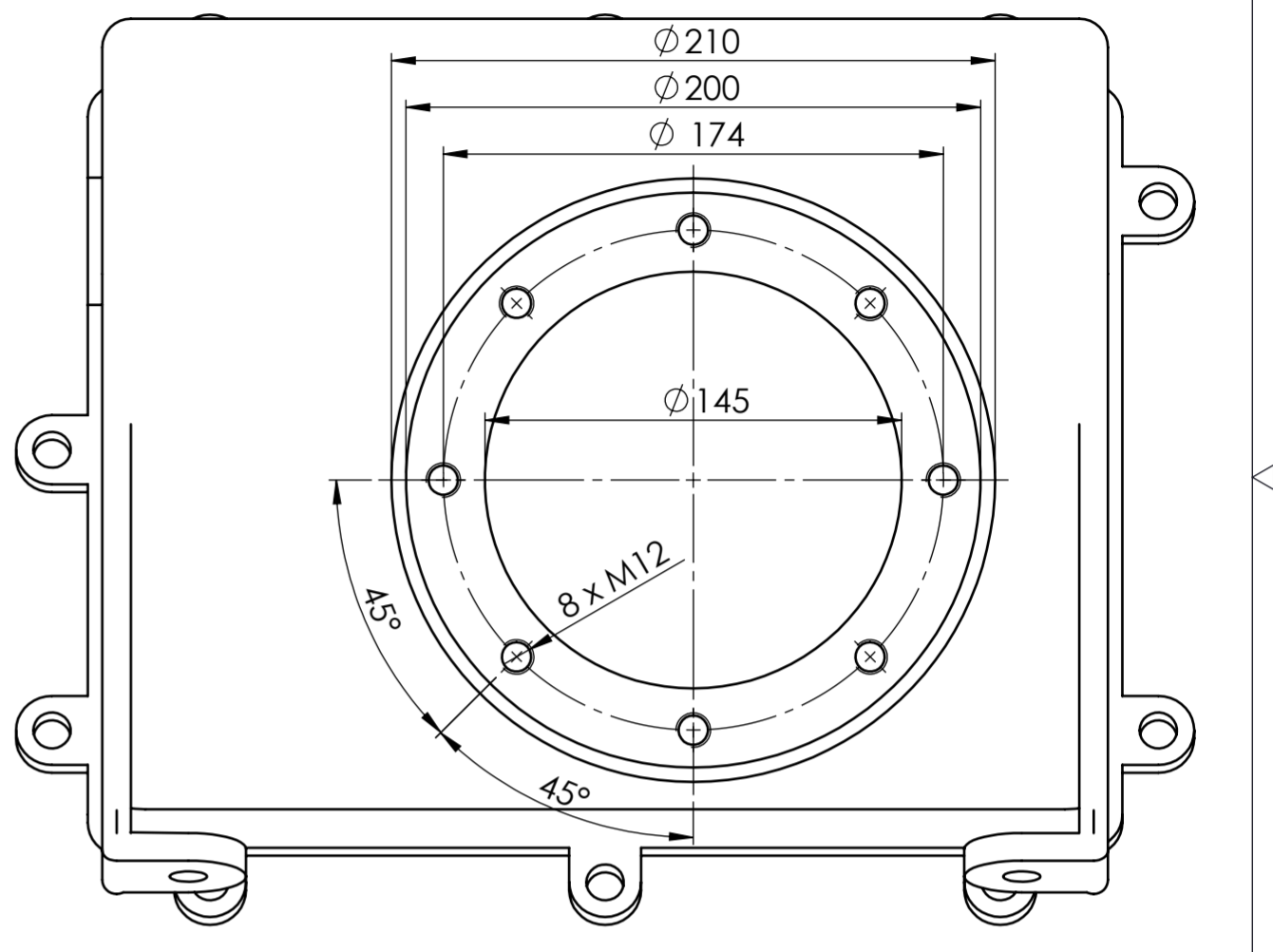
DETALJ D (1:1)
