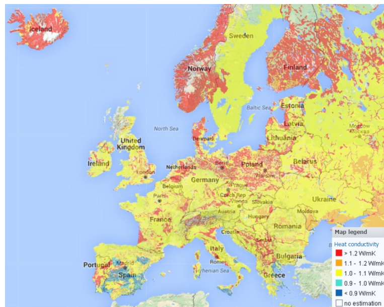
Figure 11. Map of geothermal potentials in Europe [40]
