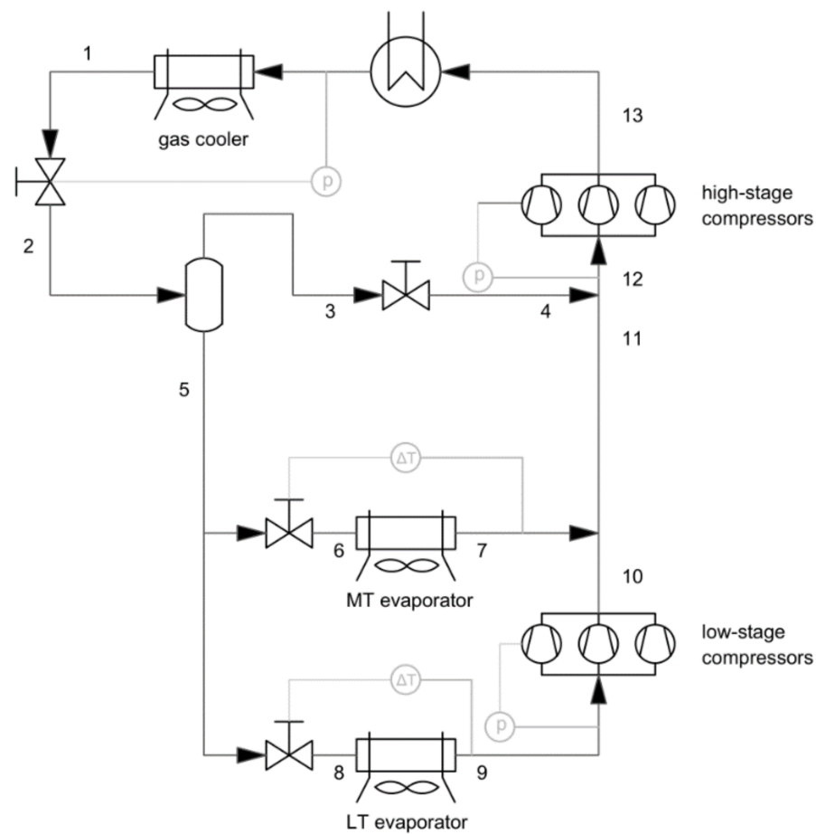
Figure 3. Scheme of CO 2 transcritical system.
