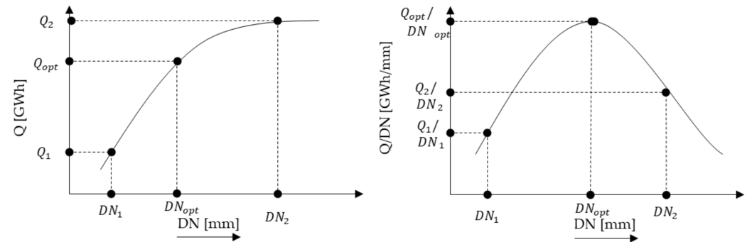
Figure 10. (Left) Utilized heat to the DH network in relation to the connection pipe diameter; (right) optimal DH network connection pipe diameter.
