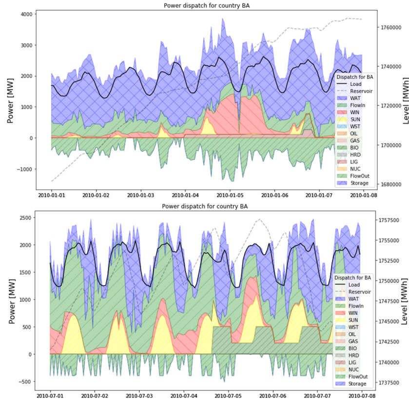
Figure 18. Weekly power dispatch curves from High RES-E 2030 scenario – Case D in January and July
