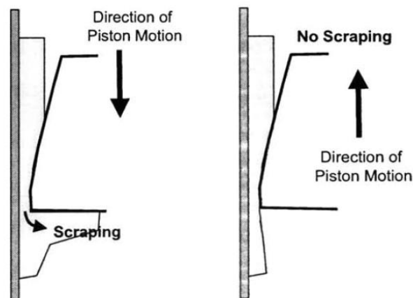
Figure 24. Effect of taper face ring profile on oil transport [11].
