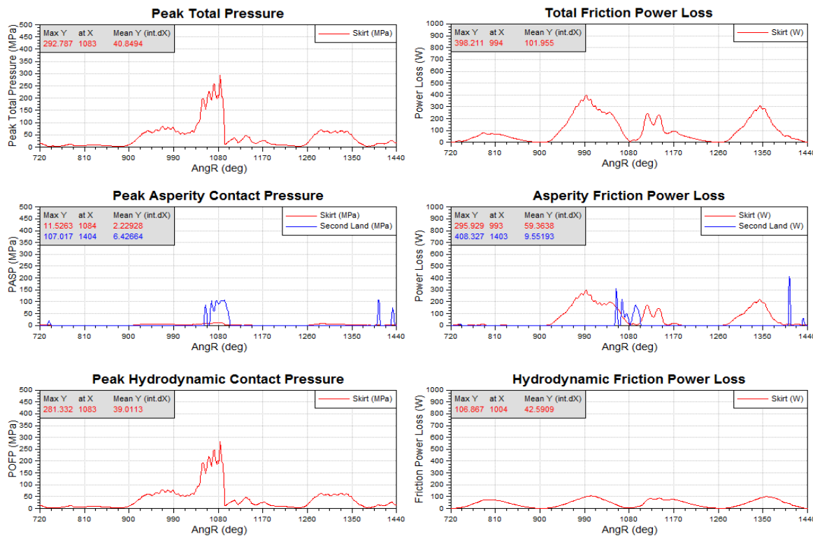
Figure D. 2. Pressure and friction results – 3000_9.3.
