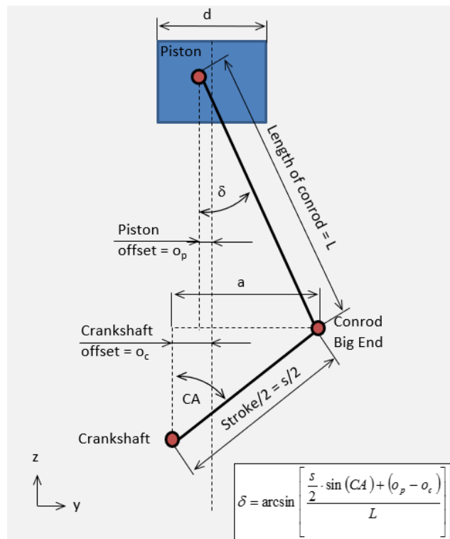
Figure 102. Dimensions necessary for calculation side force.
